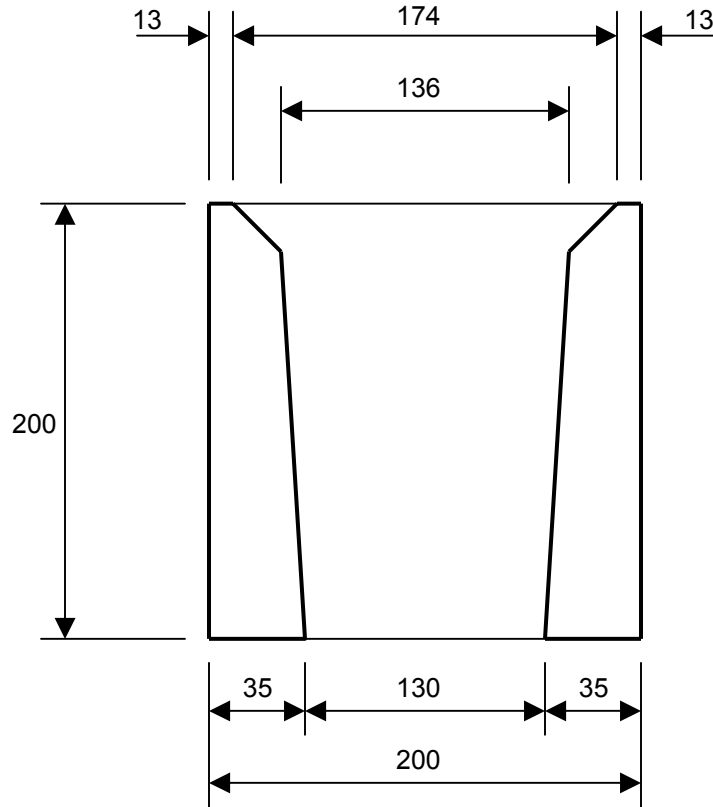
Cross Section – 200 mortarless block
